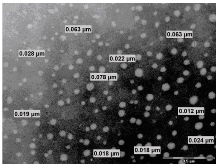
Figure 2. Transmission electron microscopic positive image of aceclofenac nanoemulsion showing the size of some oil droplets.
