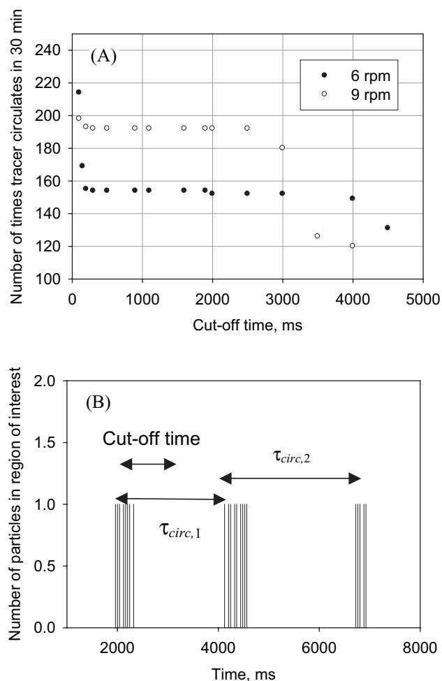
Figure 2. Estimation of cut-off time to determine circulation time. (A) typical cases for one-fourth fill at pan speeds of 6 and 9 rpm; (B) raw data for a one-eighth fill at 12 rpm for 9-mm polystyrene balls.
