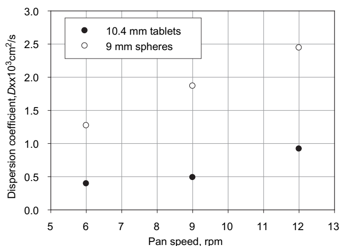
Figure 9. Comparison of dispersion coefficient (2-cm span) between 10.4-mm tablets and 9-mm spheres for one-eighth pan fill.
