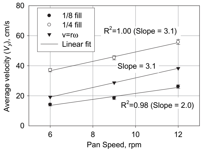
Figure 6. Average velocity parallel to the direction of flow of cascading layer as function of pan speed and pan loading for polystyrene spheres; bars, 95% confidence intervals. A linear model provides a good fit to the experimental values.
