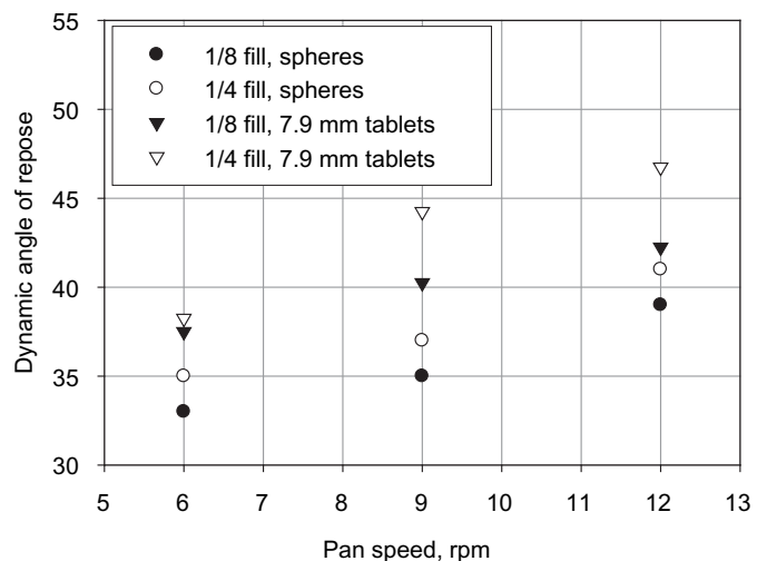
Figure 7. Dynamic angle of repose as a function of pan speed, pan loading, and particle shape.
