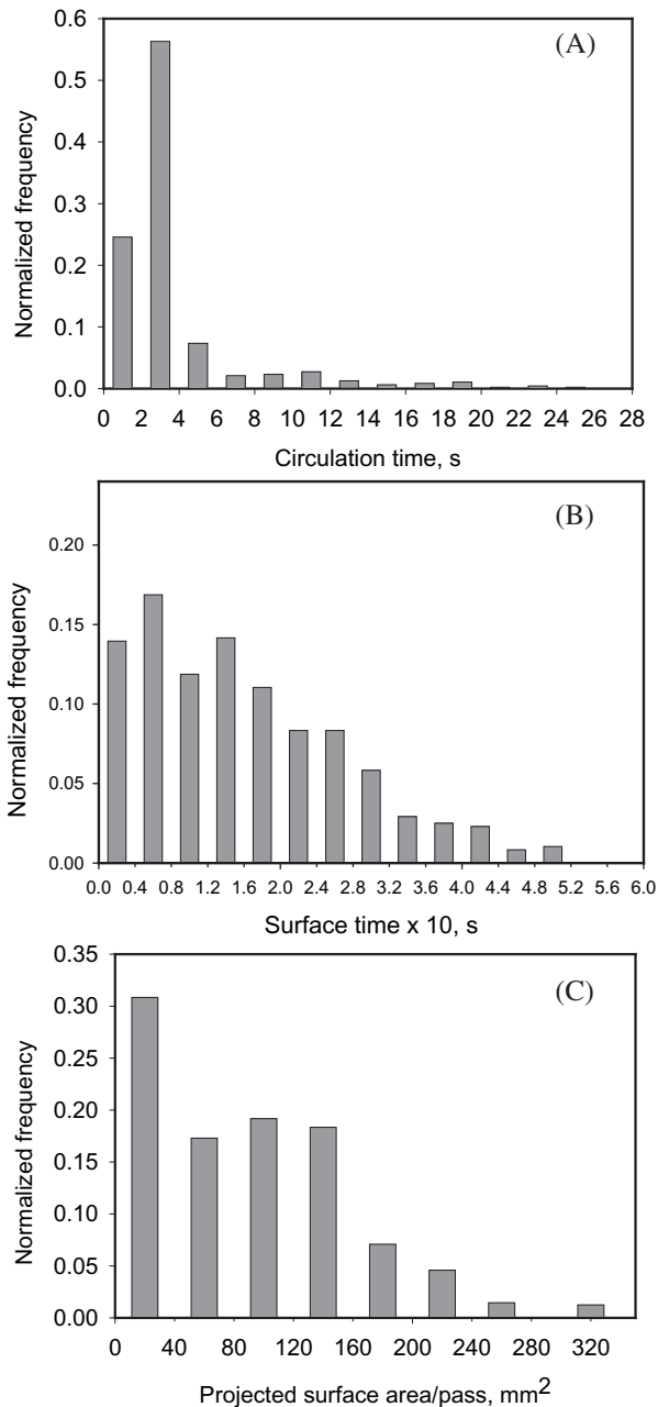
Figure 5. Distributions of (A) circulation time, (B) surface time, and (C) projected surface area per pass, at a pan speed of 9 rpm and one-eighth fill for polystyrene spheres.
