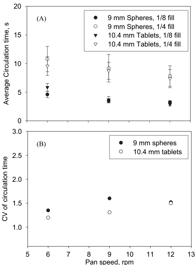
Figure 3. (A) Average circulation time as a function of pan speed and pan loading for 9-mm polystyrene spheres in comparison with 10.4-mm diameter tablets; bars, 95% confidence intervals of the average values. (B) Comparison of coefficient of variation of circulation times for 10.4-mm tablets with spheres for one-fourth fill level.
