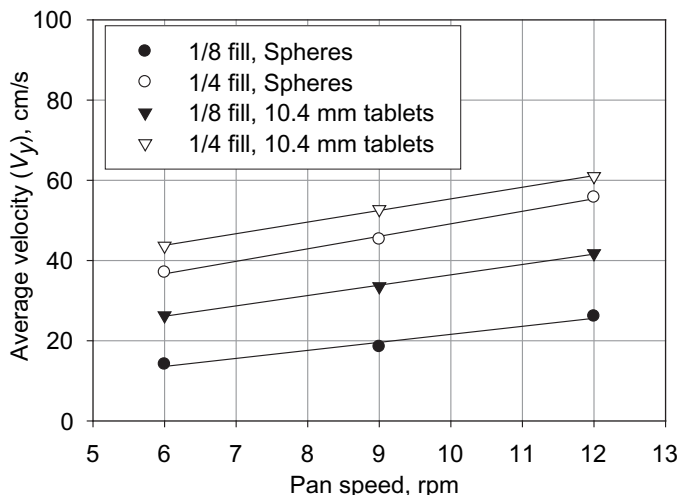
Figure 8. Comparison of average velocities in y -direction between spheres and tablets.
