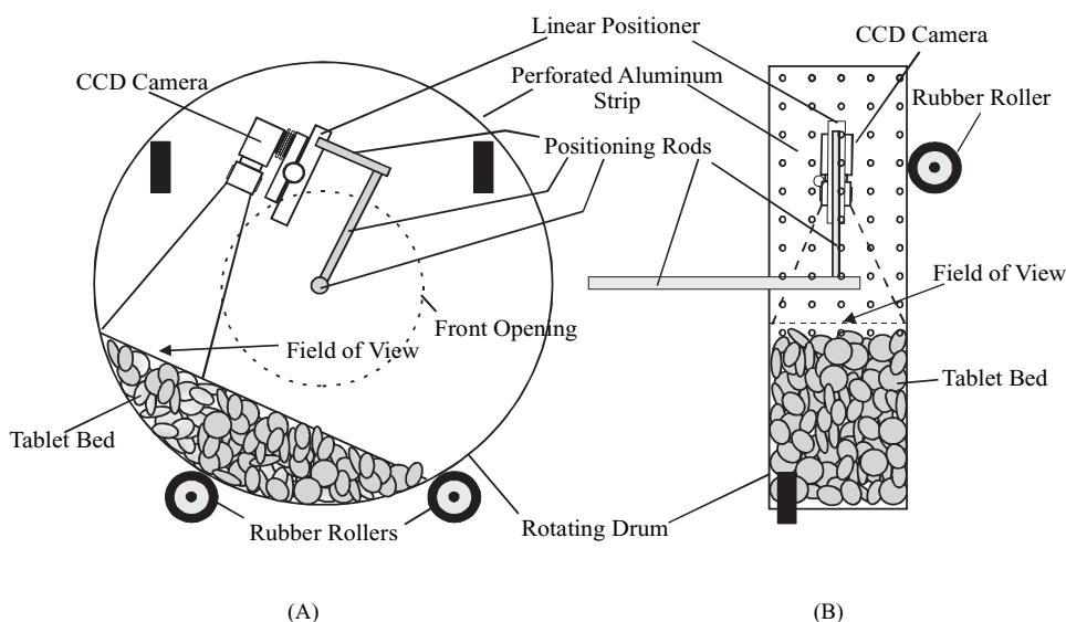
Figure 1. Experimental set-up of the 24-in pan coater used in this study. (A) side view; (B) end view. 16
