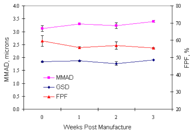
Figure 3. Effect of storage at RT on the parameters describing aerosols (MMAD \mu\text{m} , GSD, and FPF %) issued from MDIs containing lecithin inverse microemulsions in DME (100/0/2.5) ( n = 3 ).
